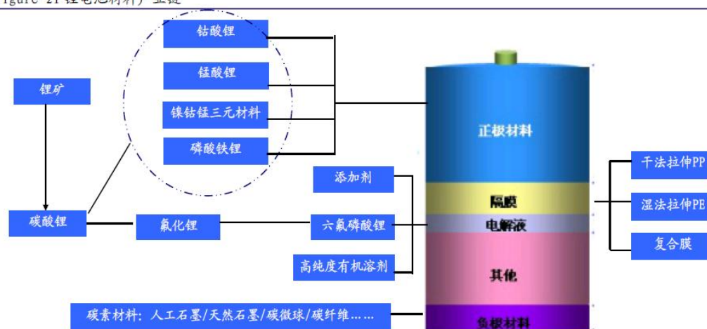
Figure 21 锂电池材料产业链
